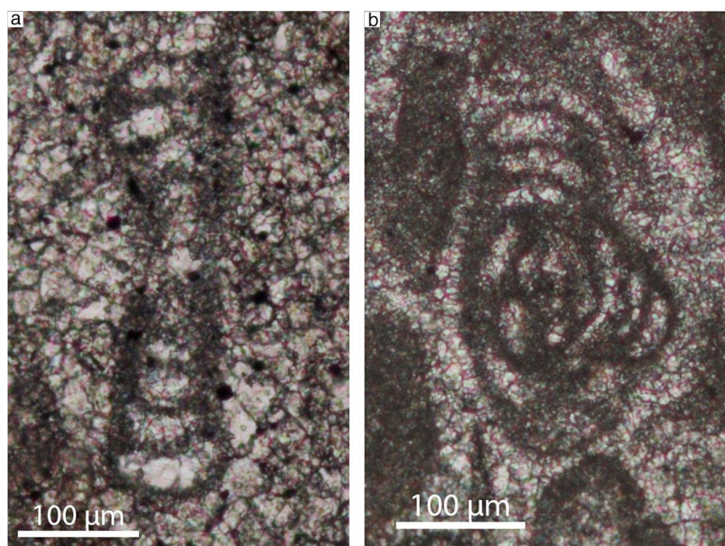
Fig. 12 Foraminifera in the Mátyáshegy Formation. (a) Ammodiscus incertus (1,000 m). (b) Hoyaella sinensis (1,145 m)
