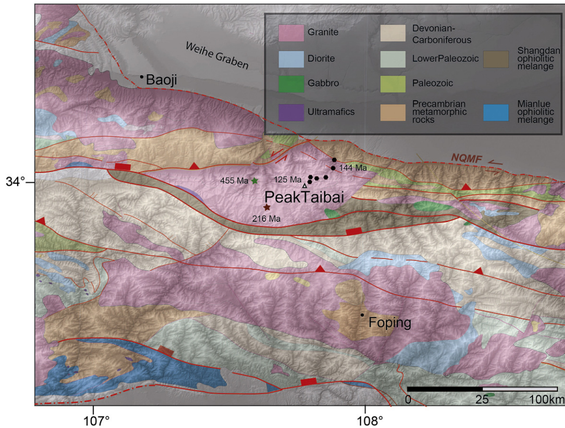
Fig. 2. Digital elevation model with superimposed geological map of the Taibai region, Qinling Mountains modified after Liu et al. (1996). Sample locations along the Taibai profile are indicated. New U–Pb data for the composite Taibai granite from this study are indicated in black, data from the literature are marked with a green (Zhou et al., 1994) and red (Xiao et al., 2000) asterisk. NQMF = North Qinling margin fault.
