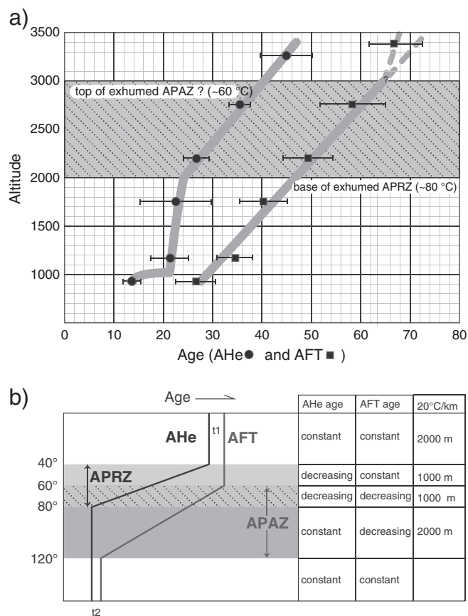
Fig. 6. a) Age-elevation correlation for apatite fission-track and apatite (U–Th–Sm)/He samples from the Taibai mountain. The break-in-slope within the AHe data at ca. 2000 m marks the onset of rapid cooling at ca. 22 to 25 Ma. A second inflection point at ca. 1000 m is interpreted as a later reheating event, probably as a result of hydrothermal fluxes. b) Concept of expected AFT and AHe ages versus depth profiles within a thermotectonically stable setting. Ages of both thermochronometers decrease simultaneously with depth where the APRZ and the APAZ overlap. T_2 marks the onset of an exhumation event, which uplifted the APRZ and APAZ; t_1 marks an older exhumation event.
