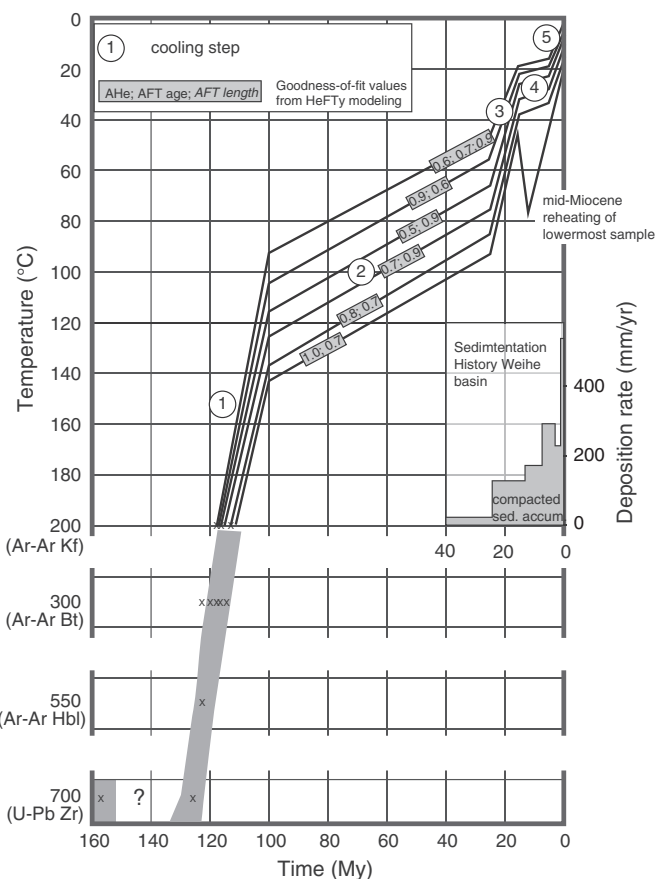
Fig. 7. Cooling history of all samples from the Taibai profile. The cooling paths are constrained by U–Pb ages, Ar–Ar ages, and forward modeling with HeFTy (Ketchum, 2005). Inset shows the sedimentation history of the Weihe graben taken from Liu et al. (2013), modified after Bellier et al. (1988a) and Xing et al. (2005). Note that the Late Oligocene–Miocene onset of intensified cooling is paralleled by an increase in sediment accumulation. Late Miocene cooling also roughly coincides with higher accumulation rates.
