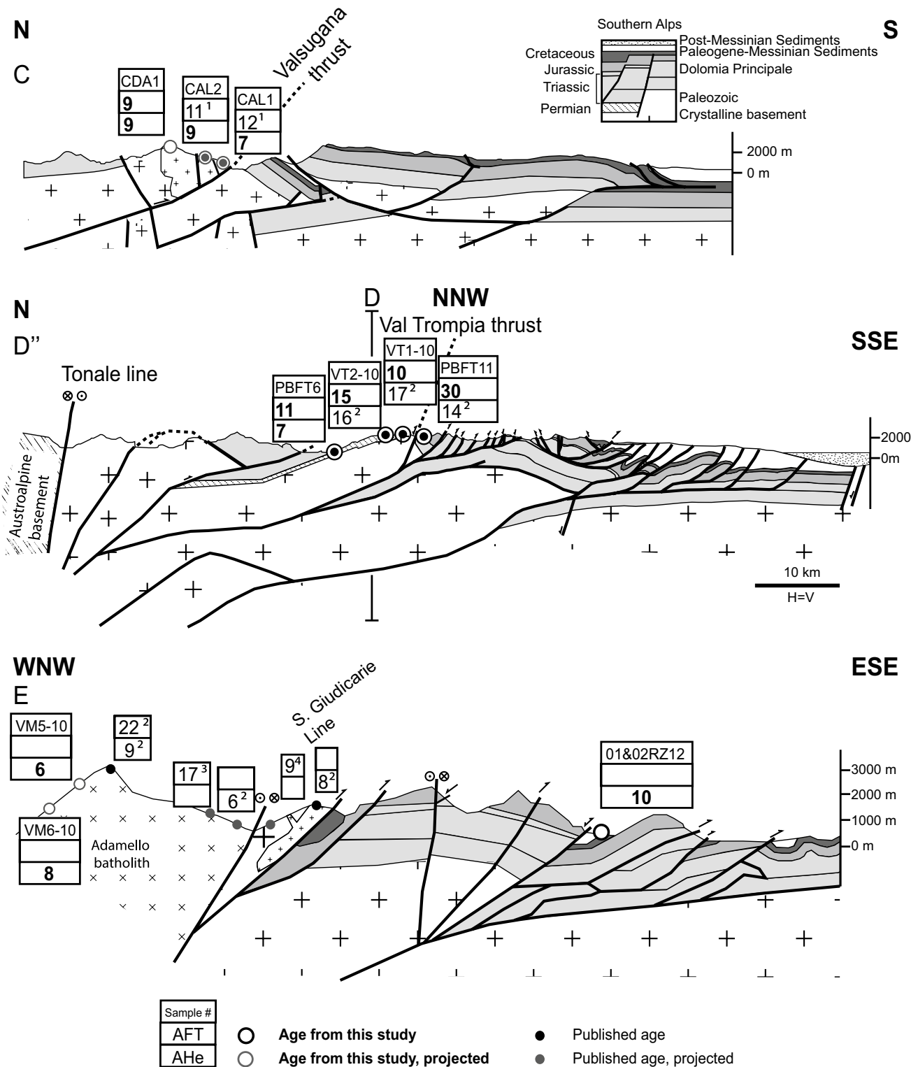
Fig. 6 Cross sections of the central Southern Alps. Section C : N–S cross section of the Valsugana thrust. Published ages are from 1 Zat-tin et al. (2003). Cross section modified after Caputo and Bosellini (1994), Selli (1998) and Barbieri and Grandesso (2007). Section D and D' : N–S and NNW–SSE cross section of the Val Trompia thrust.
