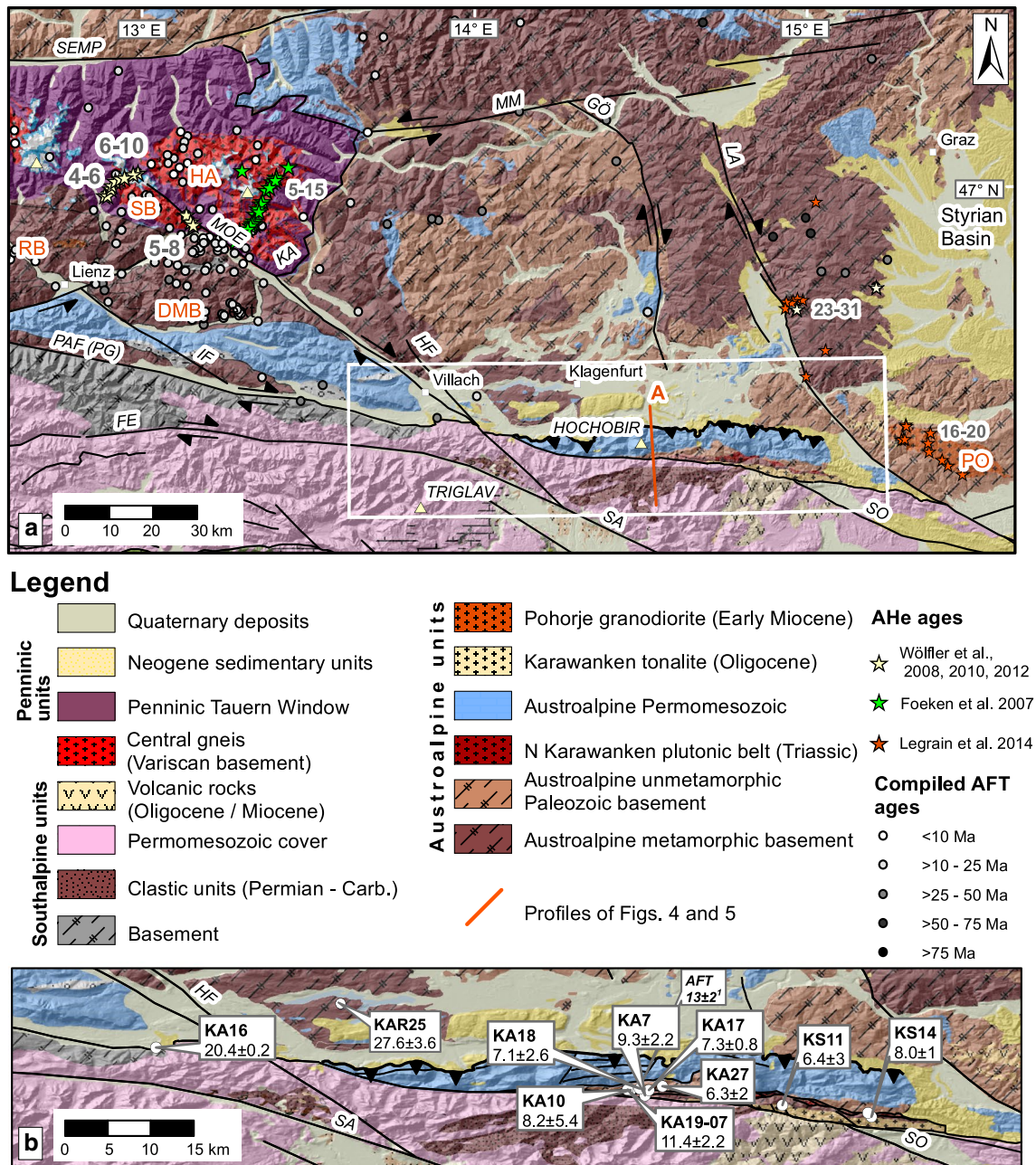
Fig. 2 a Geological map of the Eastern and Southern Alps bordering the easternmost PAF and the Karawanken Mts. illustrating major faults and summarized low-temperature thermochronology data. AFT ages were compiled from Bertrand (2013), Hejl (1997), Staufenberg (1987), Wölfler et al. (2008, 2010, 2012). DMB Drau-Möll block, FE Fella fault, GÖ Görtschitz fault, HA Hochalm-Ankogel subdome, HF Hochstuhl fault, IF Isel fault, KA Katschberg fault, LA Lavant/Labot
