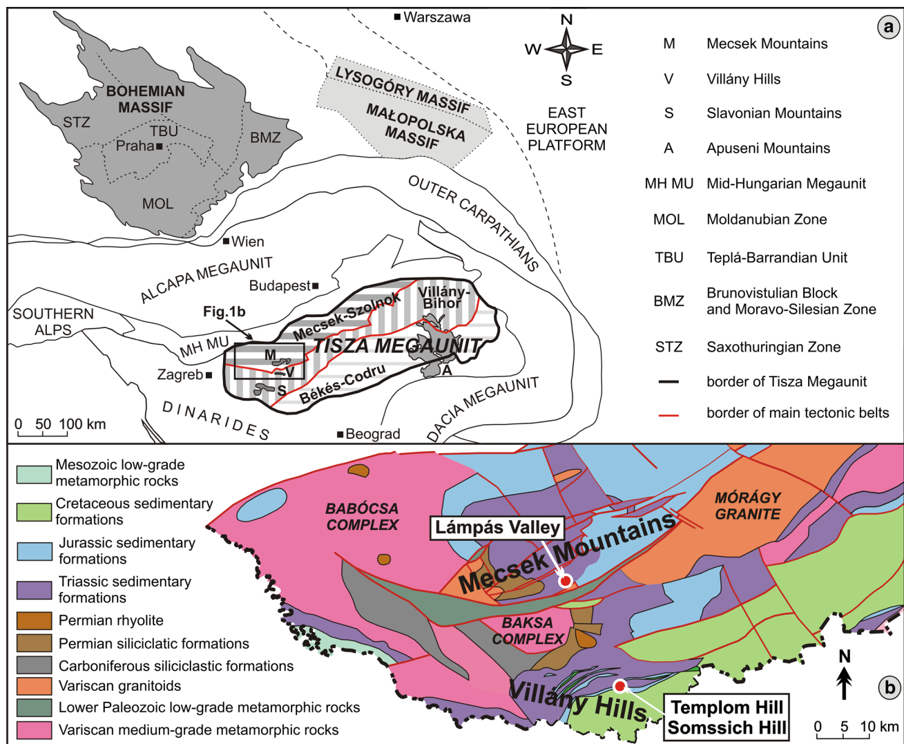
Fig. 1 a Location of the Tisza Megaunit in the Pannonian Basin and its relation to the Bohemian, Malopolska and Lysogóry Massifs (compiled after Belka et al. 2000; Haas et al. 2010; Klomínský et al. 2010; Schmid et al. 2008). b Geological sketch map of the Hungarian
