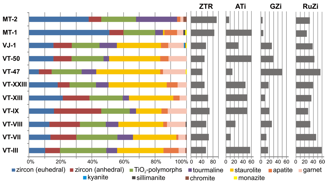
Fig. 6 Transparent heavy mineral distributions of the studied formations with the presentation of zircon–rutile–tourmaline index (ZTR index) and provenance-sensitive index values (ATi apatite–tourmaline index, GZi garnet–zircon index, RuZi rutile–zircon index)
