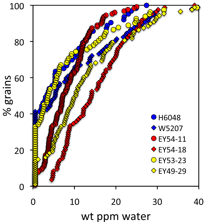
Fig. 3. Overview of the OH defect content of all samples as cumulative curves.
