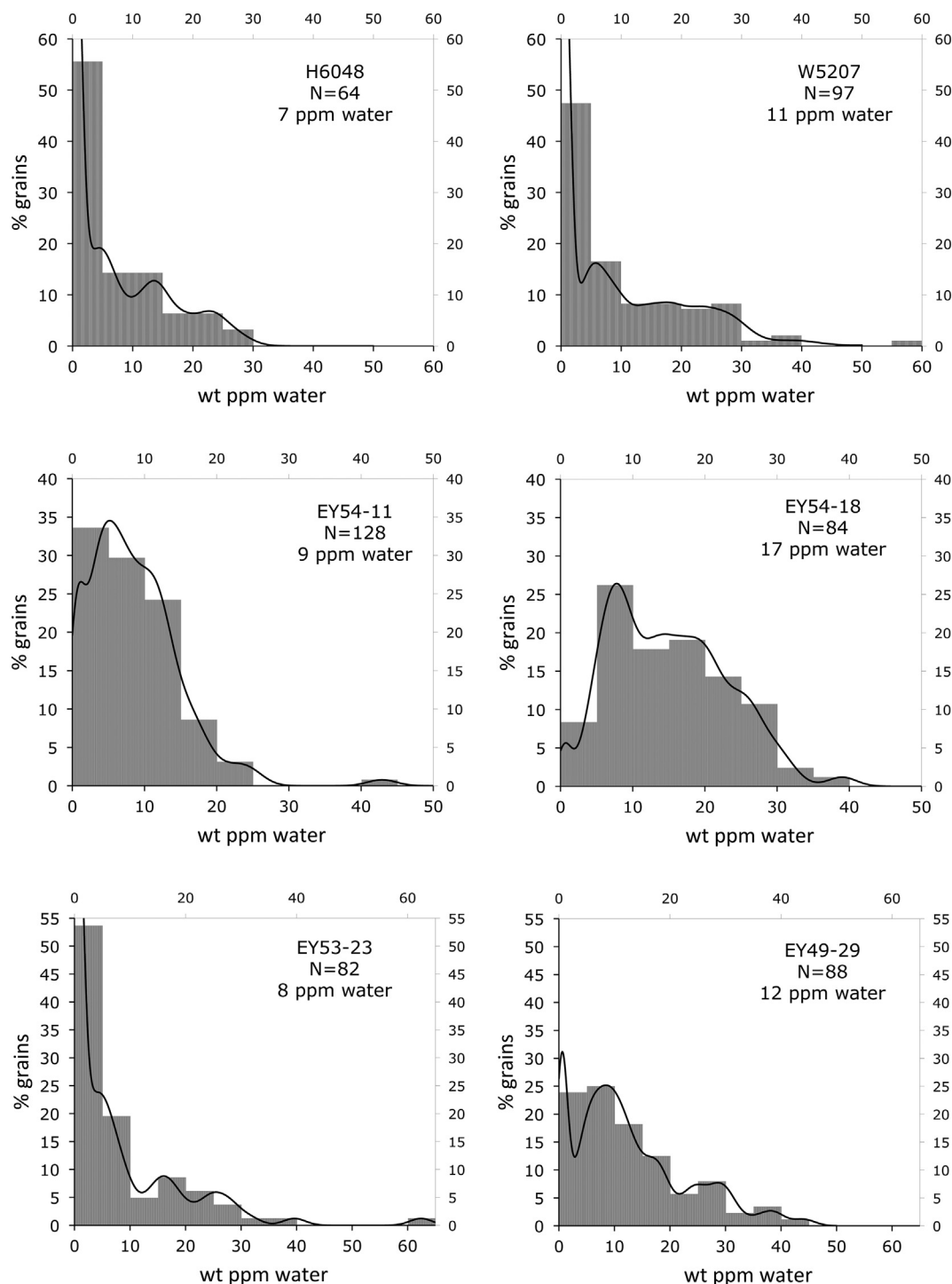
Fig. 2. Histograms showing the OH defect contents in the analysed detrital quartz grains arranged in bins of 5 ppm. The black curve indicates a weighed distribution, taking into account an error of 2 wt ppm for each single data point >2 ppm and 1 wt ppm for each data point <2 ppm defect water. Average OH defect contents and number of measured grains are displayed in each plot.
