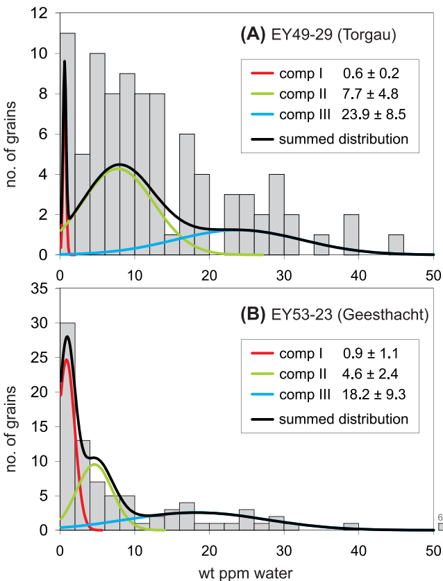
Fig. 4. Component identification according to OH defect distribution for samples EY49-29 (A) and EY53-23 (B) assuming three OH defect components each (algorithm by Dunkl and Székely, 2002): Results suggest the following component means, standard deviations (s.d.) and component percentages: (A) 0.6 \pm 0.2 ppm (5%), 7.7 \pm 4.8 ppm (66%) and 23.9 \pm 8.5 ppm (29%), (B) 0.9 \pm 1.1 ppm (39%), 4.6 \pm 2.4 ppm (30%) and 18.2 \pm 9.3 ppm (31%). For the model fitting all values below 1 ppm have been replaced by simulated values assuming normal distribution, mean of 0.5 ppm and s.d. of 1 ppm.
