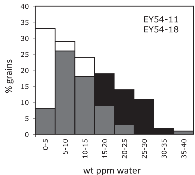
Fig. 5. Decomposition of the OH defect distribution of the two Triassic samples assuming three potential sources, one OH poor source (only in EY54-11), one common intermediate source, and one OH rich source (only in EY54-18). Distribution of sample EY54-11 (sum of white and grey bars) and EY54-18 (sum of grey and black bars) results in a relative proportion of 1:2:1, respectively. See Fig. 2 for comparison.
