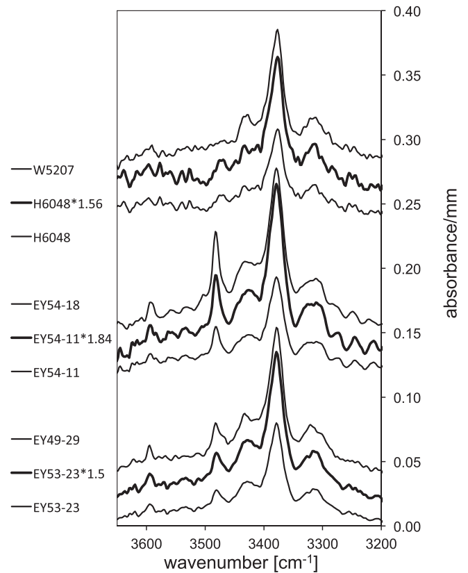
Fig. 1. Average IR spectra ( E||n_o - E||n_e ) of each sample. Bold spectra are scaled (according to the ratio of the average OH contents of the respective sample pair) in order to allow a better comparison of the band ratios of the two spectra of one succession. Spectra are normalised to 1 mm thickness and offset vertically for graphical reasons.
