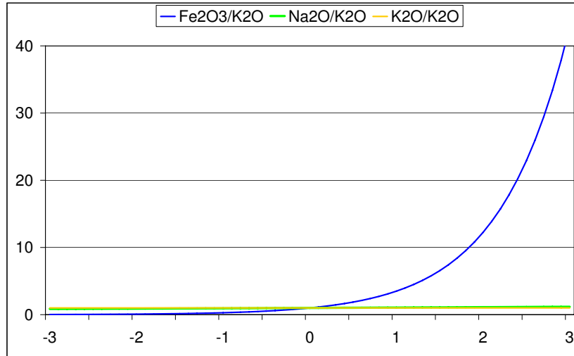
Figure 8.12: Interpretation of a principal component in \mathcal{S}^2 under the assumption of stability of K 2 O.
