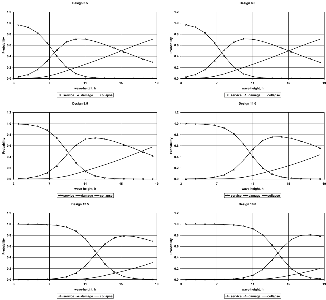
Figure 8.8: Vulnerability models obtained by regression in the simplex from the data in the Table 8.4. Horizontal axis: incident wave-height in m. Vertical axis: probability of the output response. Shown designs are 3.5, 6.0, 8.5, 11.0, 13.5, 16.0 (m design wave-height).
