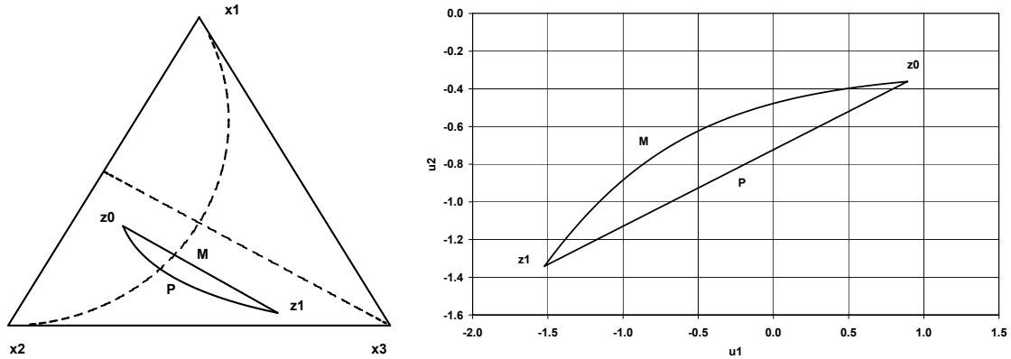
Figure 8.7: Two processes going from \mathbf{z}_0 to \mathbf{z}_1 . (M) mixture process; (P) linear perturbation process. Representation in the ternary diagram, left; using balance-coordinates u_1 = 6^{-1/2} \ln(z_1 z_2 / z_3) , u_2 = 2^{-1/2} \ln(z_1 / z_2) , right.
