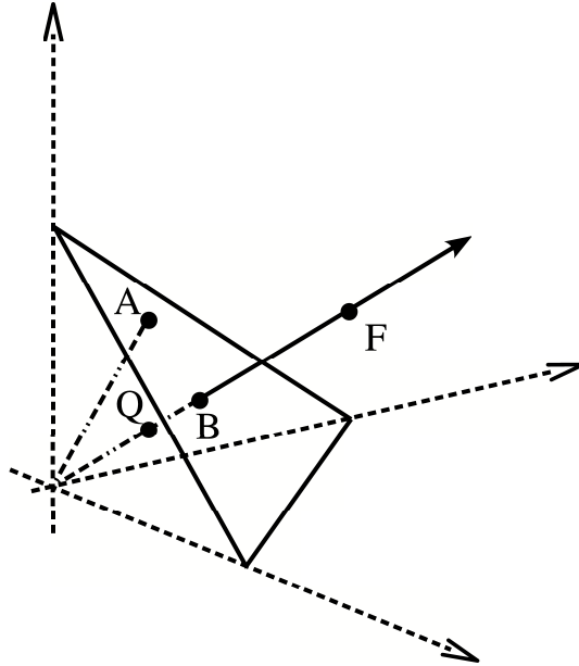
Figure 2.2: Representation of the compositional equivalence relationship. A represents the original sandstone composition, B the final sand composition, F the amount of each part if feldspar was added to the system (first hypothesis), and Q the amount of each part if quartz was depleted from the system (second hypothesis). Note that the points B, Q and F are compositionally equivalent.
