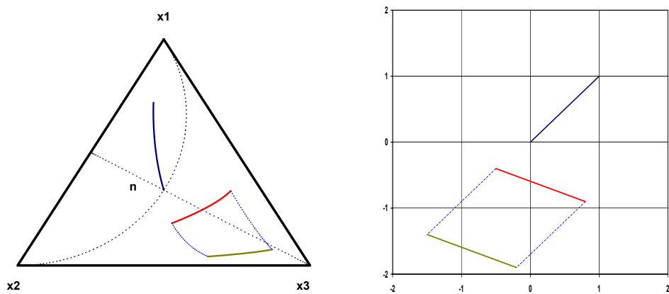
Figure 4.1: Perturbation of a segment in \mathcal{S}^3 (left) and in coordinates (right).
