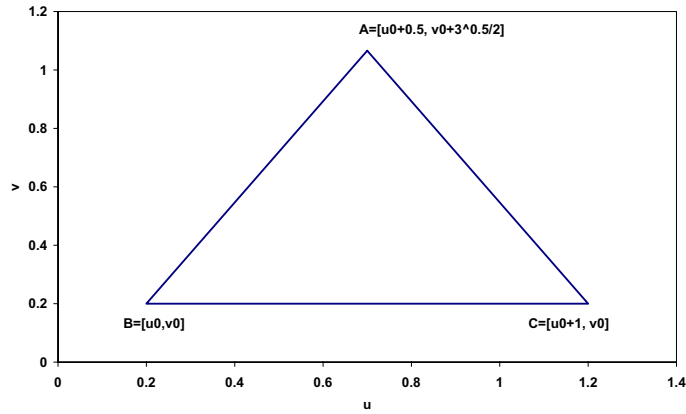
Figure 13: Plot of the frame of a ternary diagram. The shift plotting coordinates are [u_0, v_0] = [0.2, 0.2] , and the length of the side is 1.
