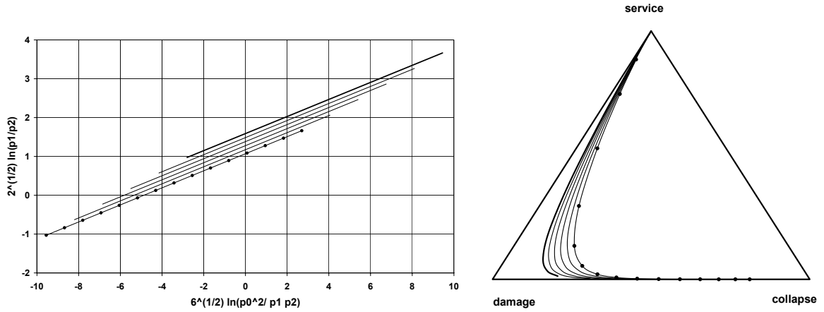
Figure 8.9: Vulnerability models in Figure 8.8 in coordinates (left) and in the ternary diagram (right). Design 3.5 (circles); 16.0 (thick line).
