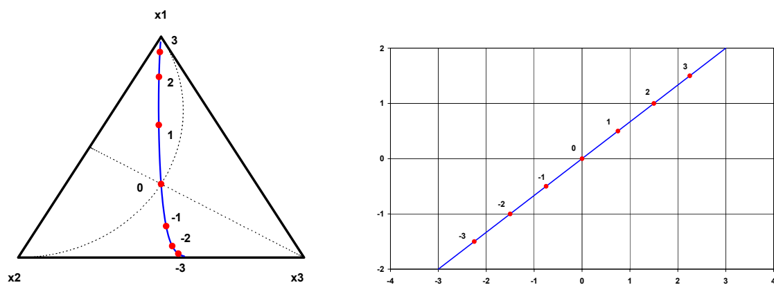
Figure 4.2: Powering of a vector in \mathcal{S}^3 (left) and in coordinates (right).
