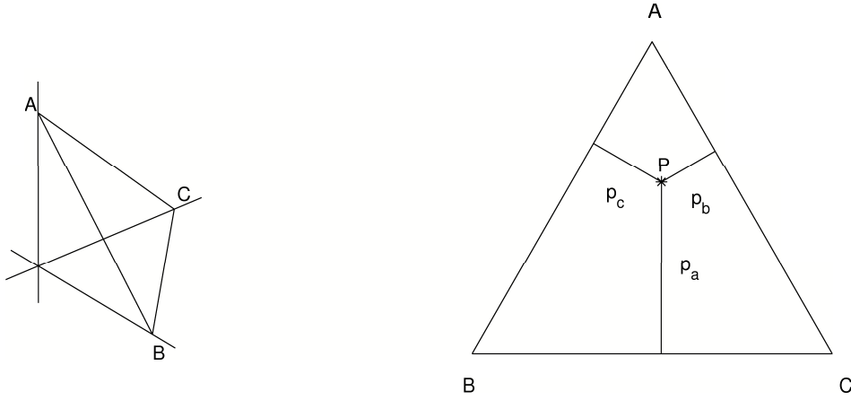
Figure 2.1: Left: Simplex imbedded in \mathbb{R}^3 . Right: Ternary diagram.
