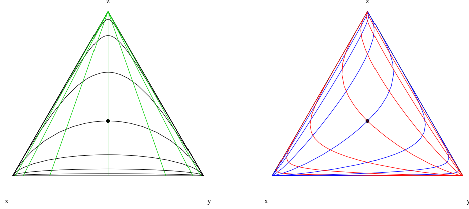
Figure 3.2: Orthogonal grids of compositional lines in \mathcal{S}^3 , equally spaced, 1 unit in Aitchison distance (Def. 3.5). The grid in the right is rotated 45^\circ with respect to the grid in the left.
