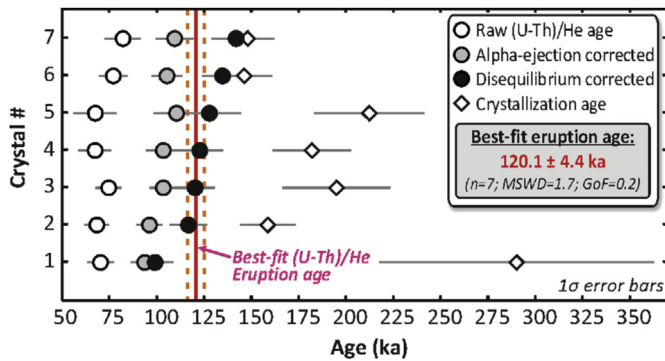
Fig. 3. An example of eruption age calculation from (U-Th)/He and U-Th-disequilibrium ages and the effect of F_t and disequilibrium corrections on final eruption age calculated using MCHCalc (Schmitt et al., 2010b). Data adopted from Schmitt et al. (2011) (sample ALA-4); uncertainties of 1\sigma are shown for clarity. Note the effect of magma residence time on magnitude of the disequilibrium correction for individual crystals.
