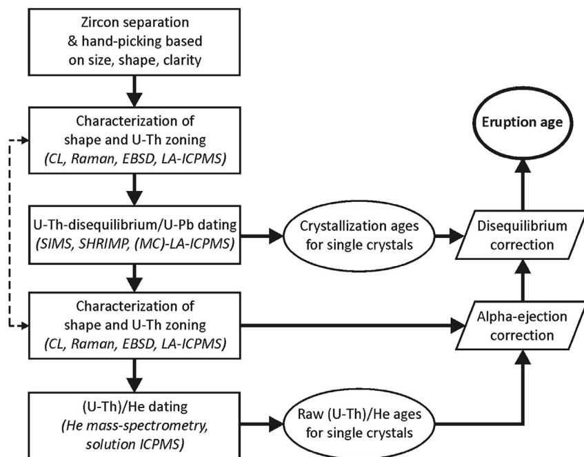
Fig. 2. Flow chart showing steps recommended for combined U-Th-disequilibrium/U-Pb and (U-Th)/He dating. Note that characterization of zircon crystals for U-Th distribution and physical dimensions required for F_t correction can be undertaken before or after the U-Th-disequilibrium/U-Pb dating step.
