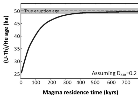
Fig. 1. The effect of magma residence time (x-axis) on measured (U-Th)/He age. The curve is calculated for a zircon crystal with true eruption age of 50 ka by assuming D_{230} = 0.2 which is a typical value for zircon (Charlier and Zellmer, 2000; Farley et al., 2002). The grey band is a typical analytical uncertainty for the (U-Th)/He method. Note that ignorance of a disequilibrium effect may result in underestimation of the age by up to 50% for crystals with short magma residence times. Also note that after >300 kyrs of magma residence, the effect of disequilibrium on (U-Th)/He may not be detectable.
